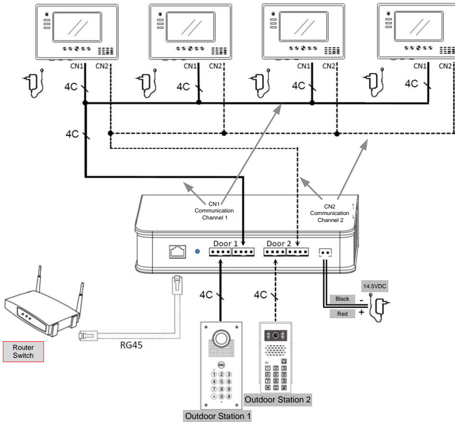
Figure 2 - Conception Cloud Server System Integration- 2 Outdoor Station Systems
