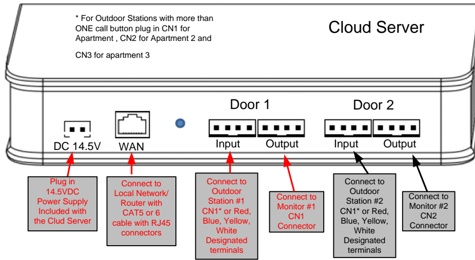
Figure 1- Connectors View
